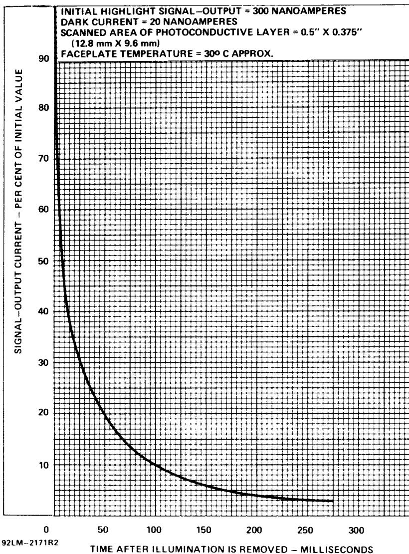
Figure 4 – Typical Persistence Characteristics
