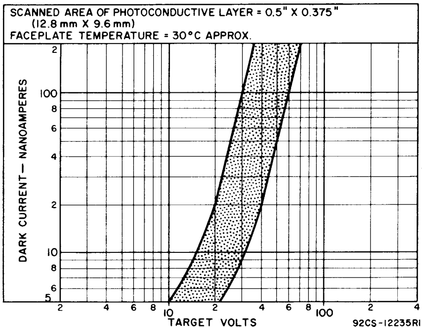
Figure 3 — Range of Dark Current
