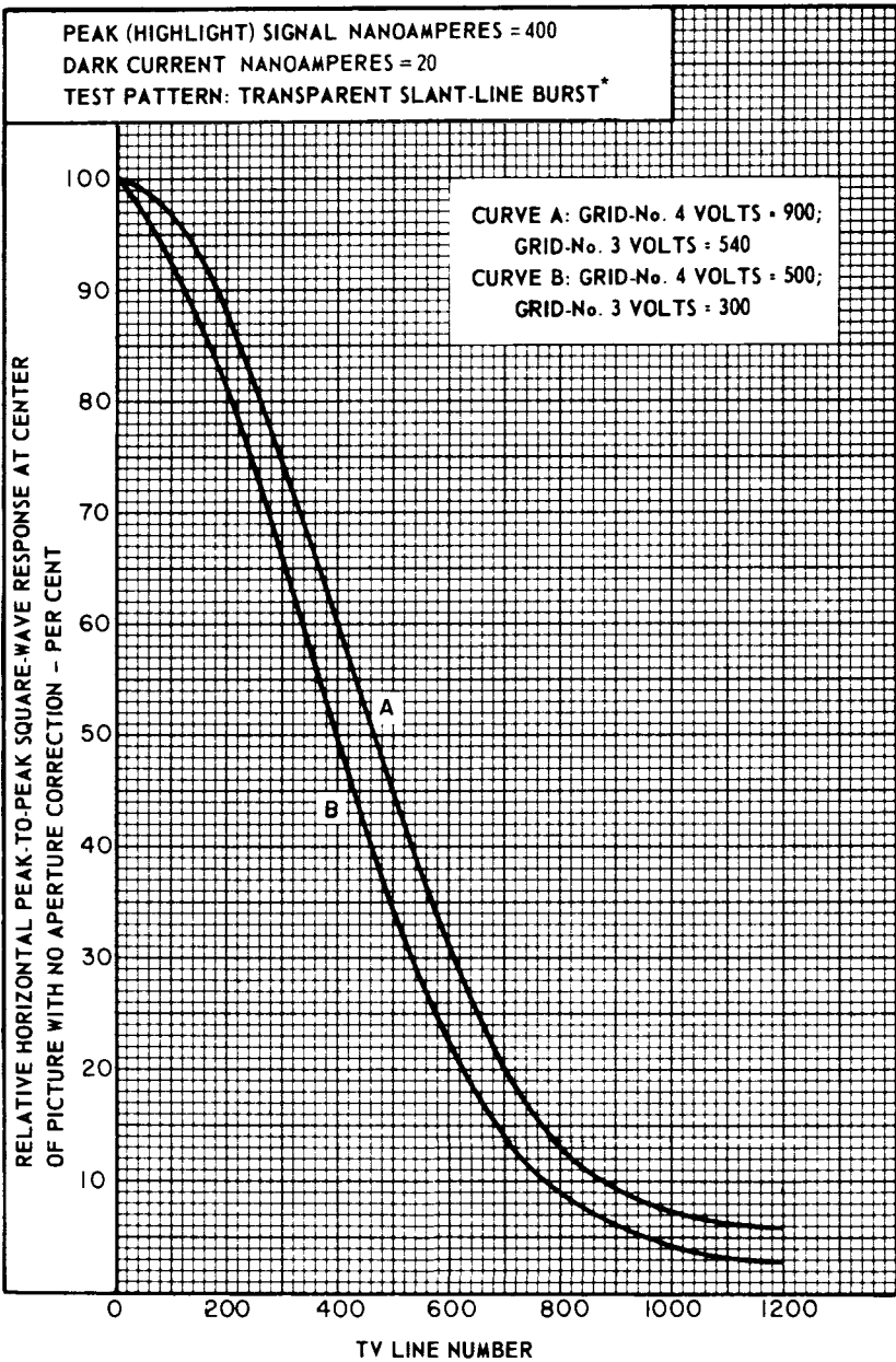
Figure 6 — Horizontal Square-Wave Response
