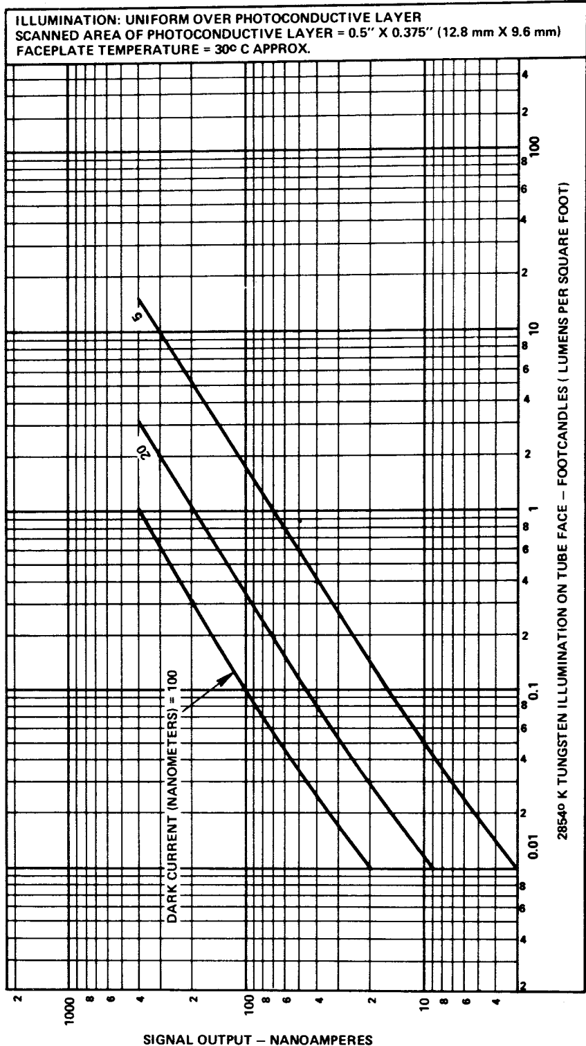
Figure 7 – Light Transfer Characteristics
