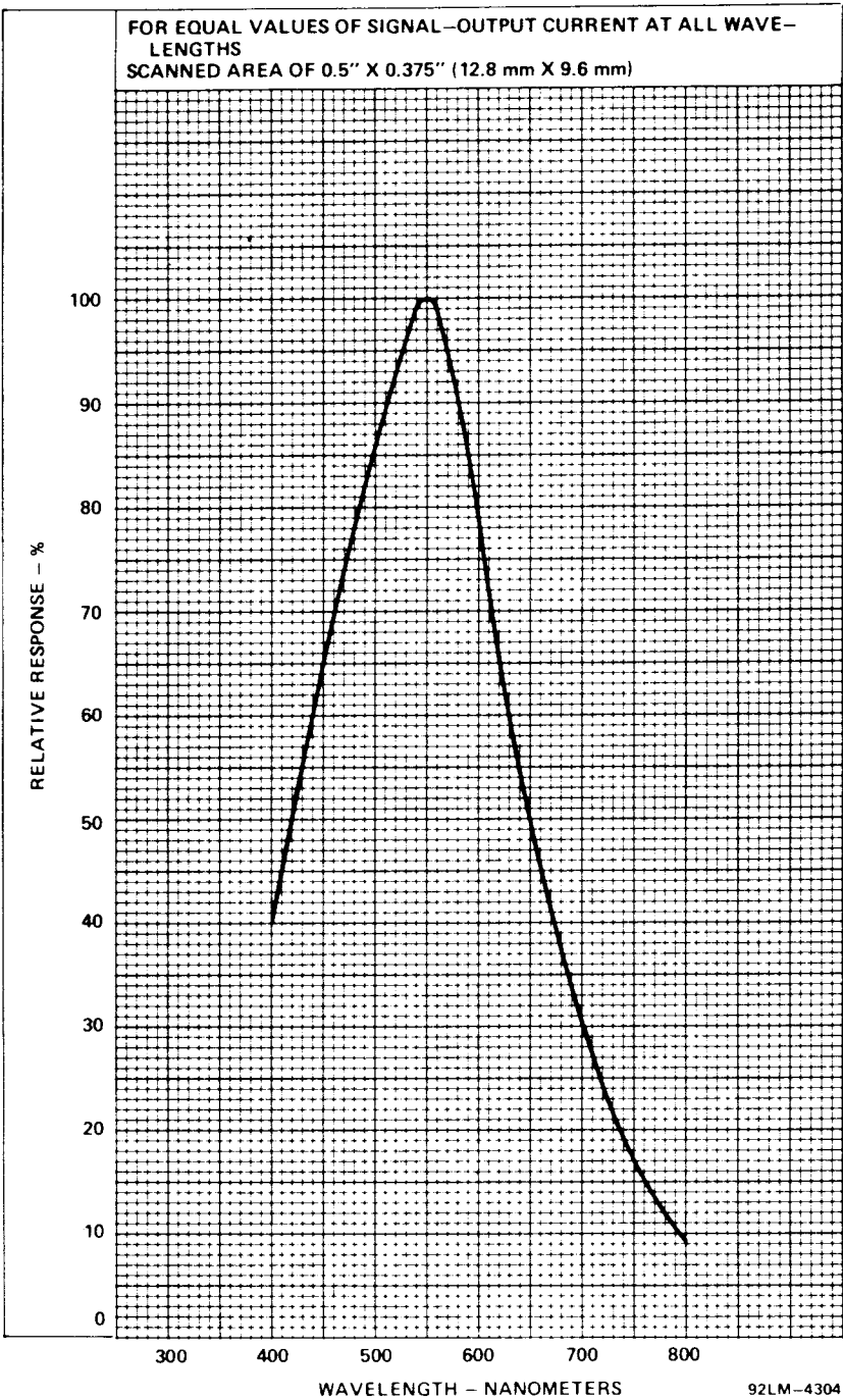
Figure 5 — Typical Spectral Response
